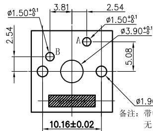
P.C.B mounting detail General Tolerance: ±0.05
