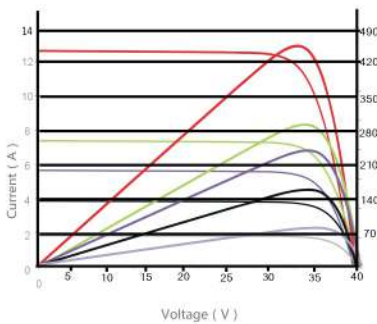
Current-Voltage & Power-Voltage Curves (435W)
