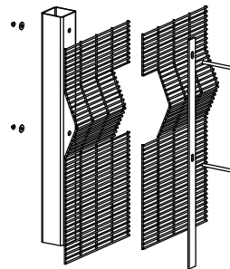
POST FIXING DETAIL
