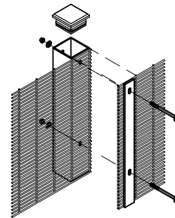
POST FIXING DETAIL
