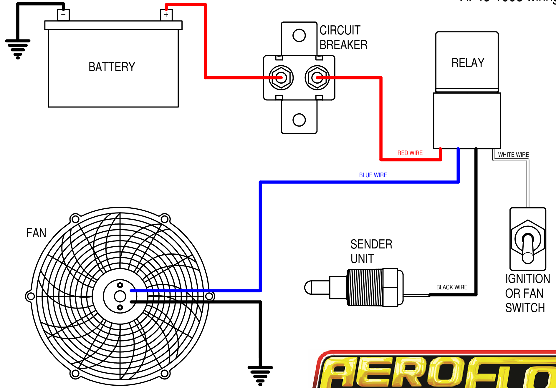
AF49-1006 wiring diagram
