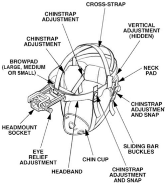
Figure 2-2 Headmount Diagram
