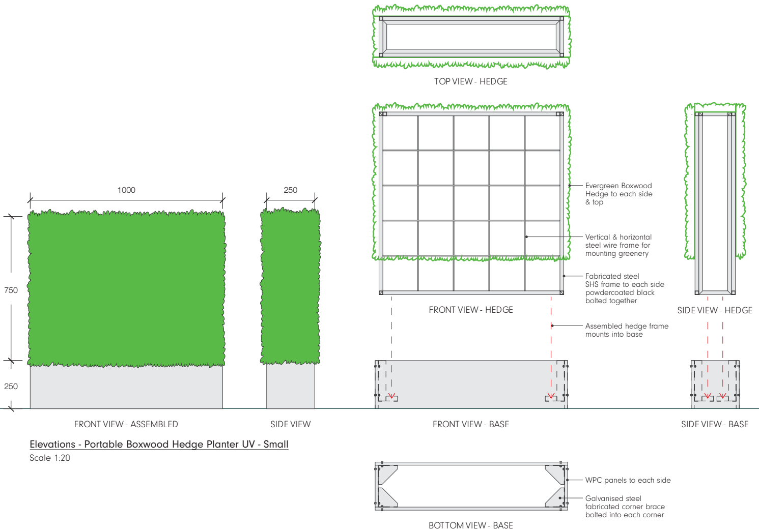
Elevations - Portable Boxwood Hedge Planter UV - Small - Components
