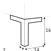
no. 47 metal chrome, painted black
