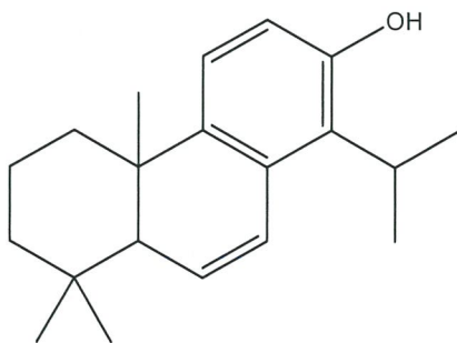
6,7-dehydro totarol
