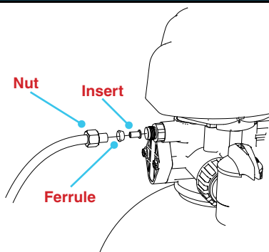
BRINE LINE CONNECTION TO CONTROL VALVE
