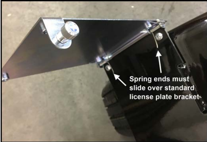
Photo: SOLPH placed on trailer with spring ends slid over bracket
