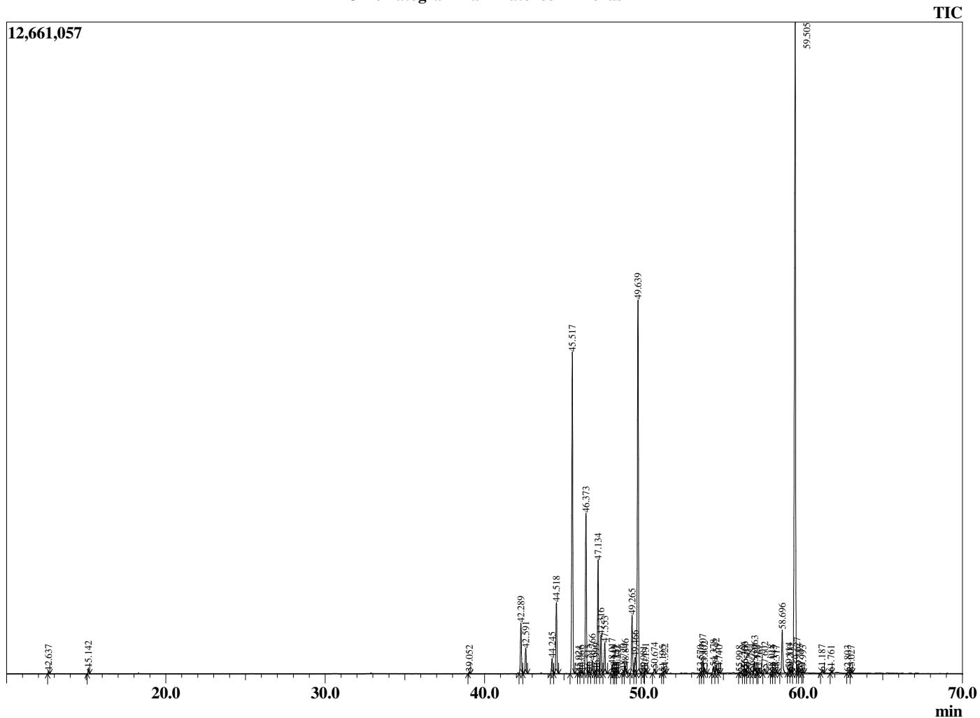
Chromatogram Dark Patchouli - Helias
