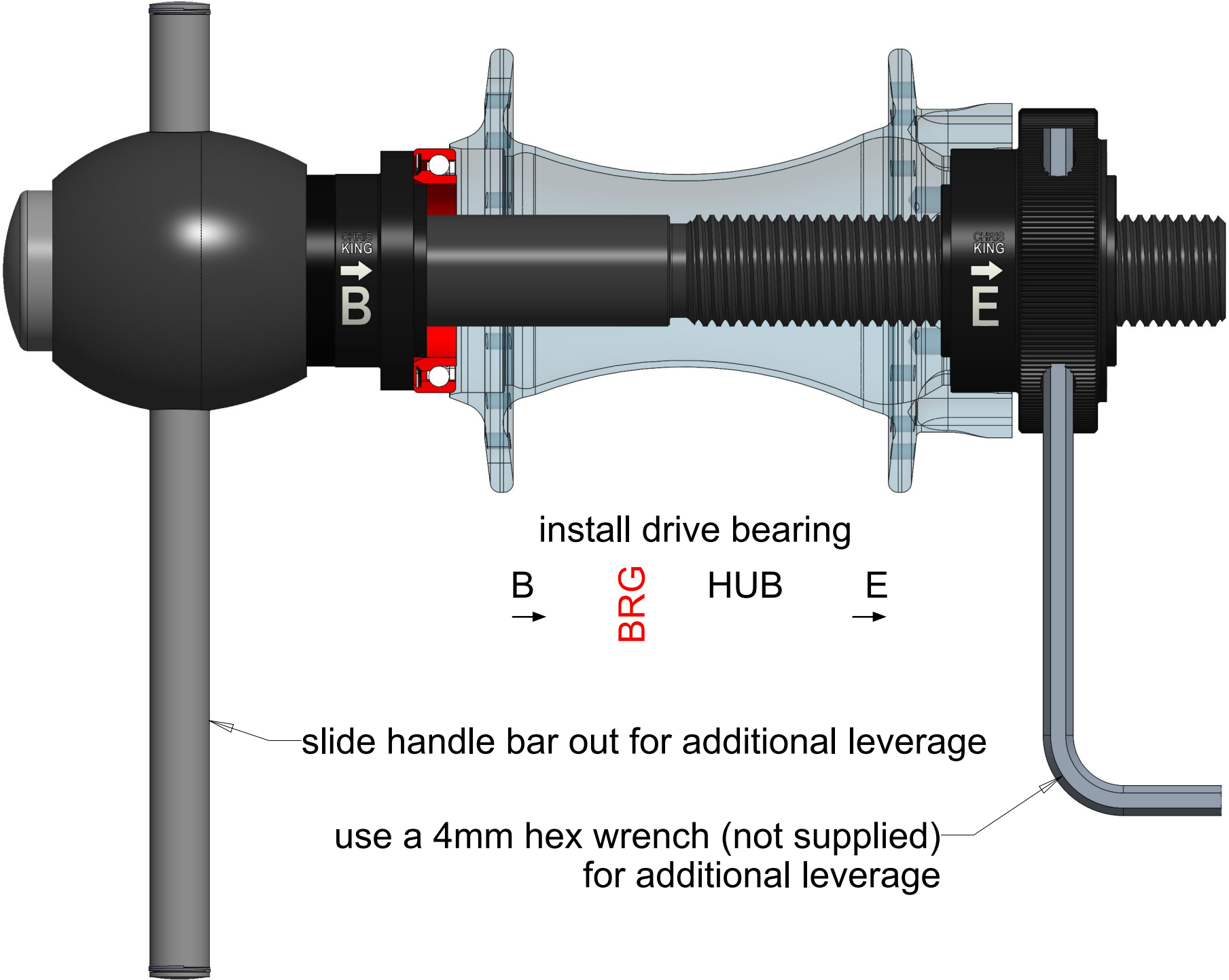
FIGURE 7 INSTALLING FRONT HUB DRIVE BEARING EXAMPLE
