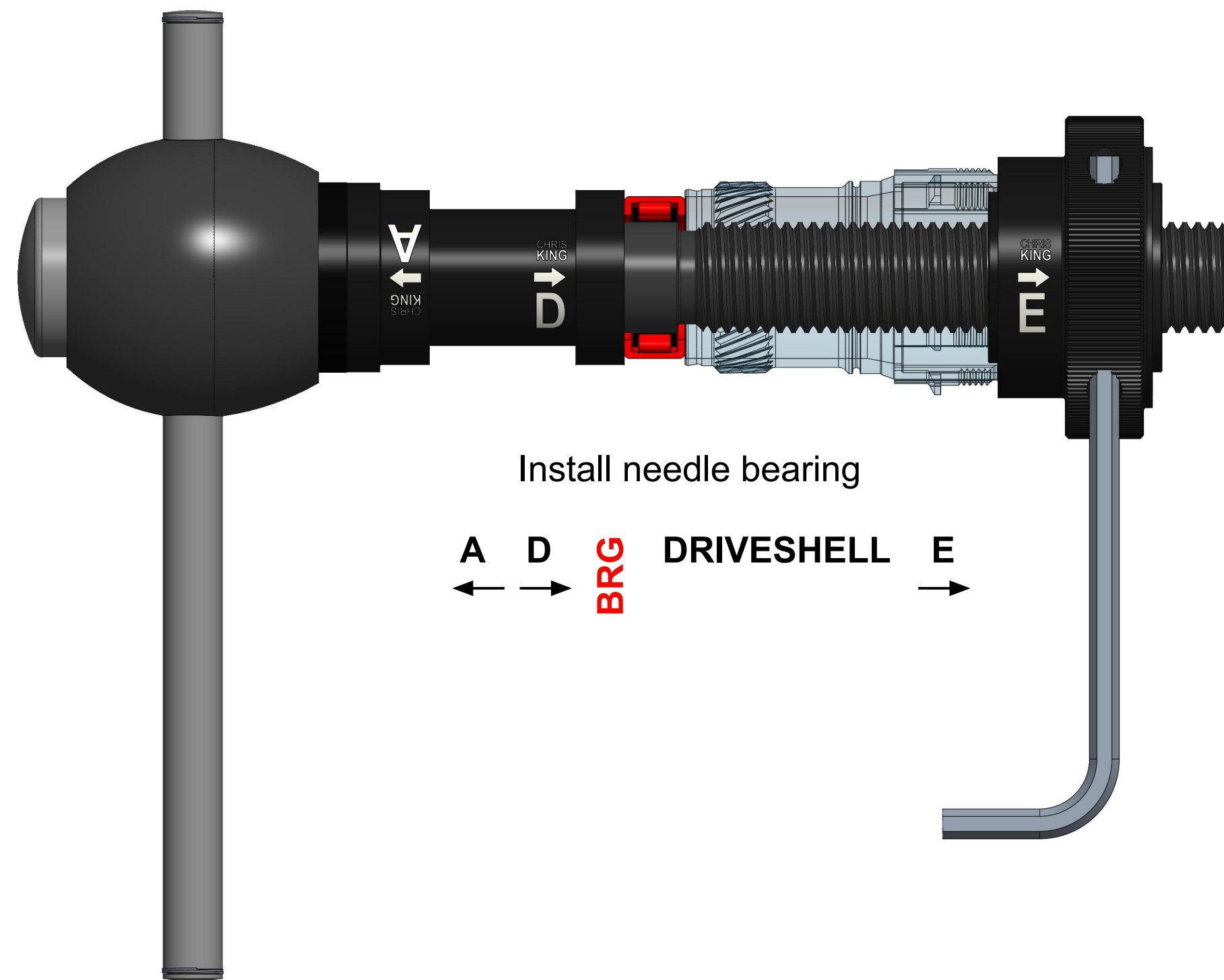
FIGURE 15 INSTALL BMX DRIVESHELL NEEDLE BEARING
