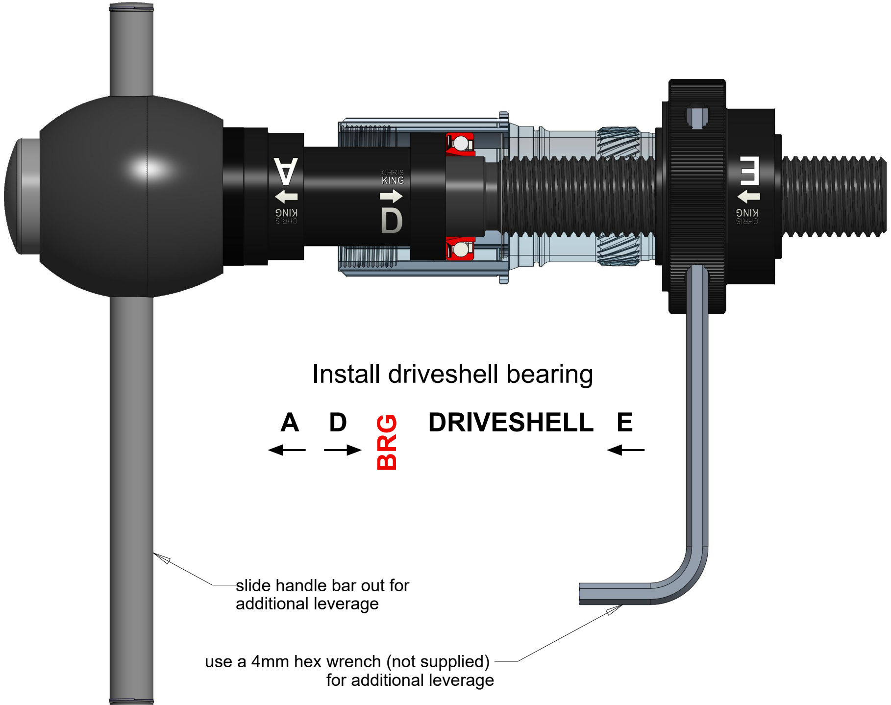
FIGURE 13 INSTALL DRIVESHELL BEARING EXCEPT BMX NEEDLE BEARING
