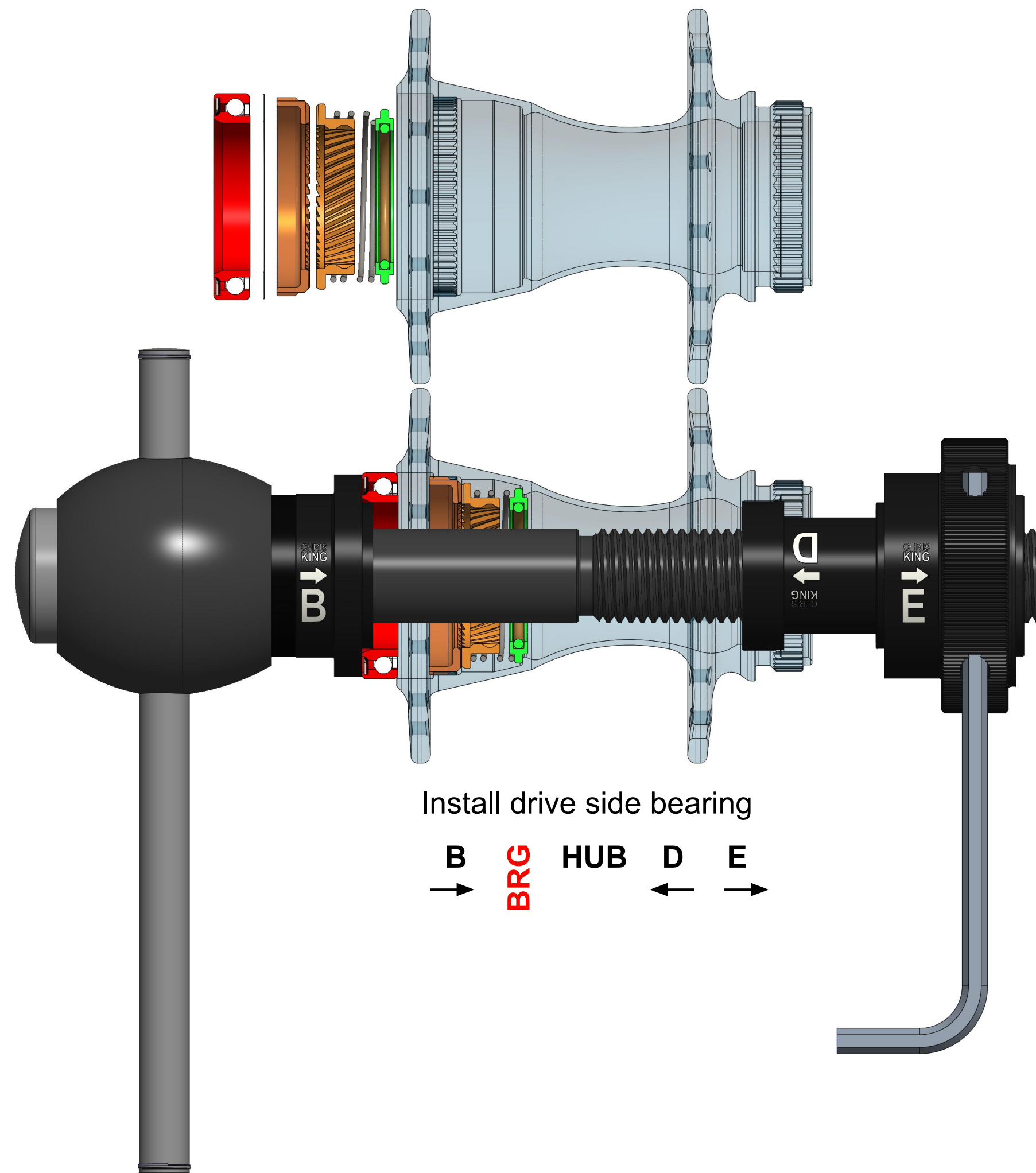
FIGURE 10 INSTALLING REAR HUB DRIVE SYSTEM AND BEARING R45 AND R45D
