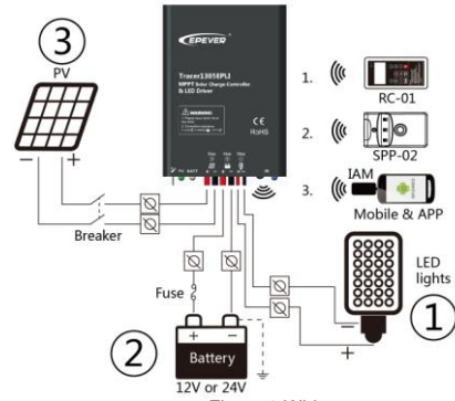
Figure 3 Wiring
