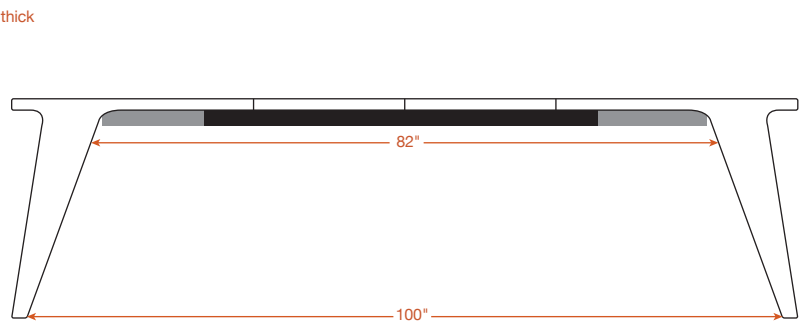
FRONT (open w/ 2 leaves)
