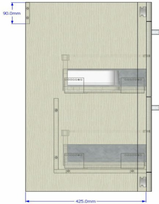
Left Elevation
