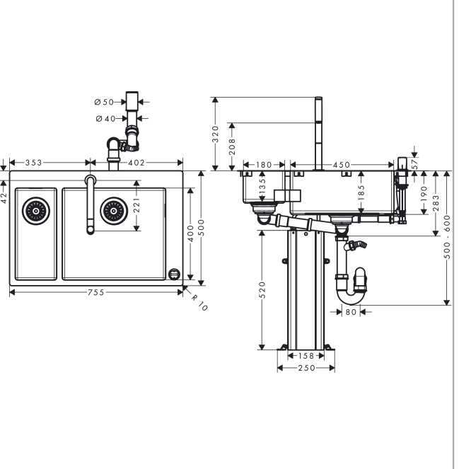
Scale drawing
