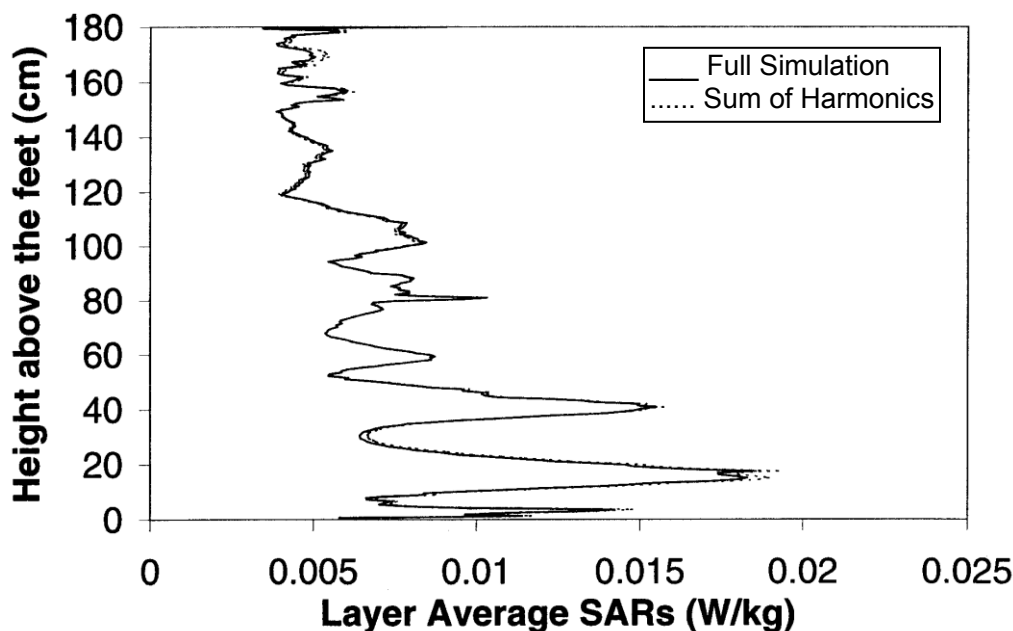
Figure 1-6. The calculated layer-averaged SAR distribution for the model of the human body due to a base station antenna made of an 18-cm-tall vertical dipole in front of a flat reflector of dimensions 24 x 24 cm. Frequency = 835 MHz, radiated power = 10 W, distance to the front plane of the model = 2 m.
