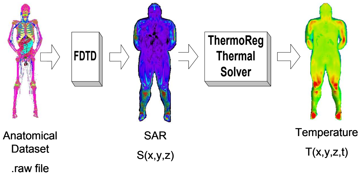
Figure 6-2. An heterogeneous tissue data set (“ .raw file ”) is used as the geometry in the FDTD calculations to determine local SAR values. The same raw file, along with the calculated SAR data, is used to determine local tissue temperatures over time using the ThermoReg finite difference thermal solver.
