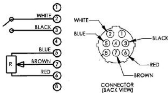
Wiring Diagram C850-0815X Foot Control
