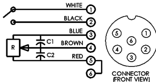
Wiring Diagram – C810-0625
