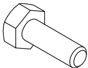
HEX BOLT 1/4"-20 x 3/4" UNC Gr8 Qty 8
