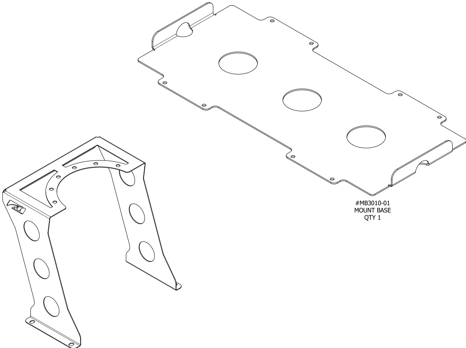
#MB3010-02 MOUNT STRAP QTY 2
