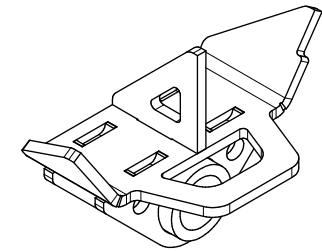
SHACKLE HANGER, PASSENGER QTY 1
