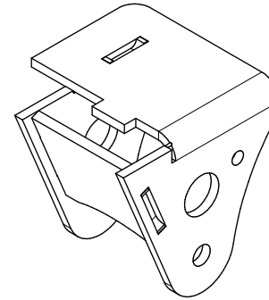
SPRING BUCKET, DRIVER QTY 1
