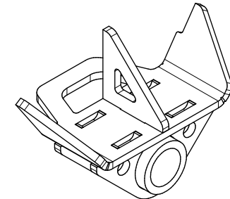
SHACKLE HANGER, DRIVER QTY 1
