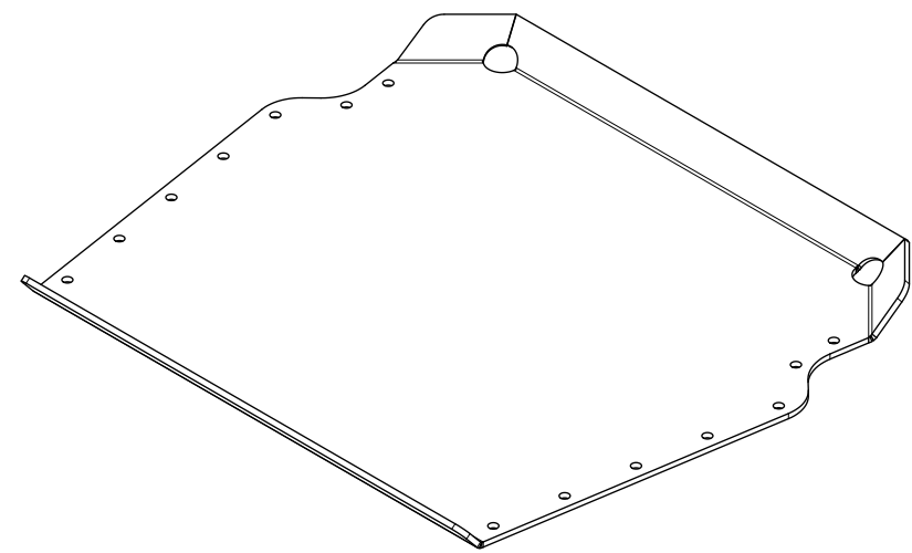
#MB1517-15 SKID PLATE QTY 1
