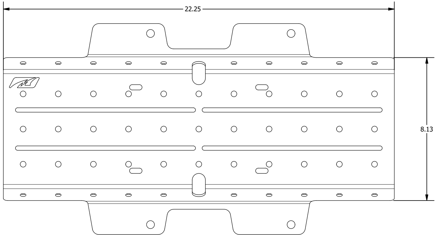
#MB1116 TAILGATE ACCESSORY MOUNT QTY 1
