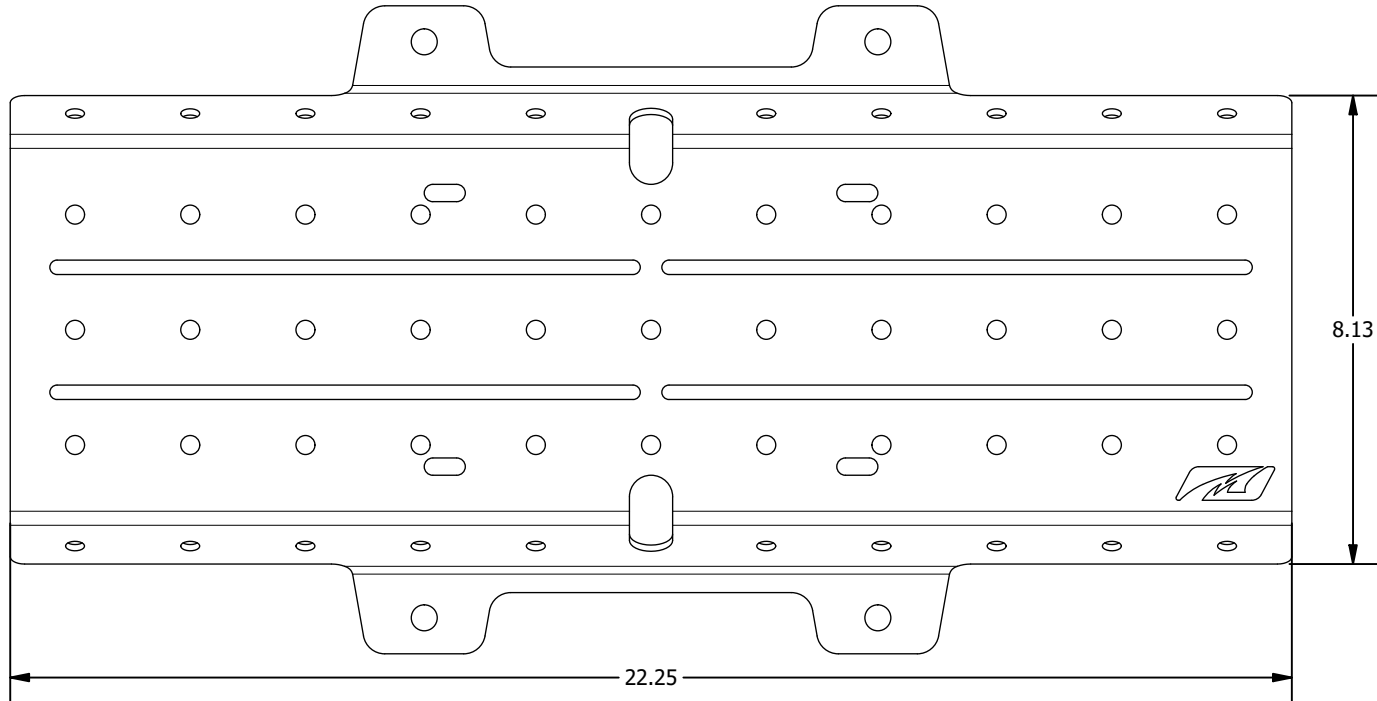
#MB1115 ACCESSORY MOUNT QTY 1
