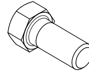
HEX BOLT 7/16"-14 x 1.0, Gr 8 QTY 4
