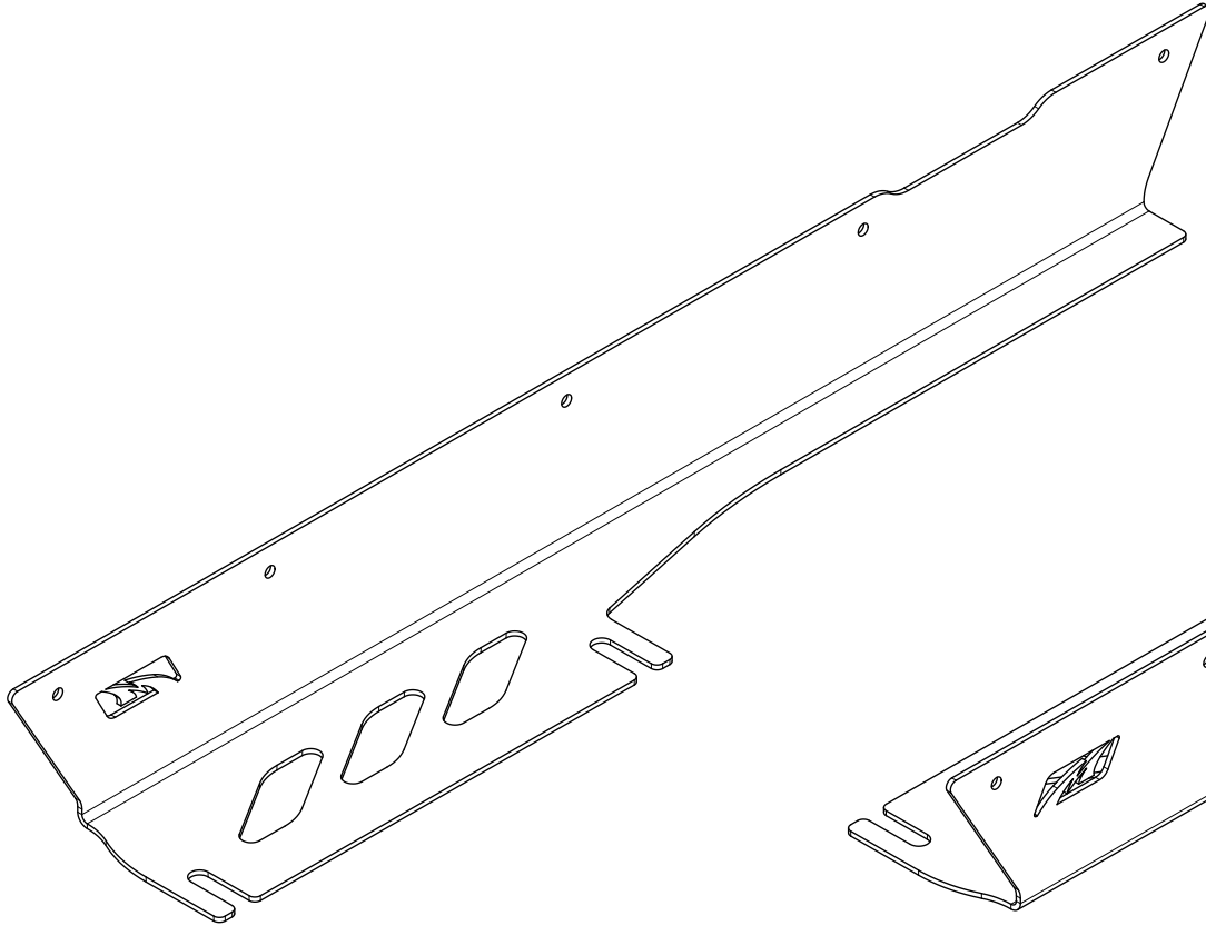
#MB1059-01 PASSENGER ROCKER GUARD QTY 1
