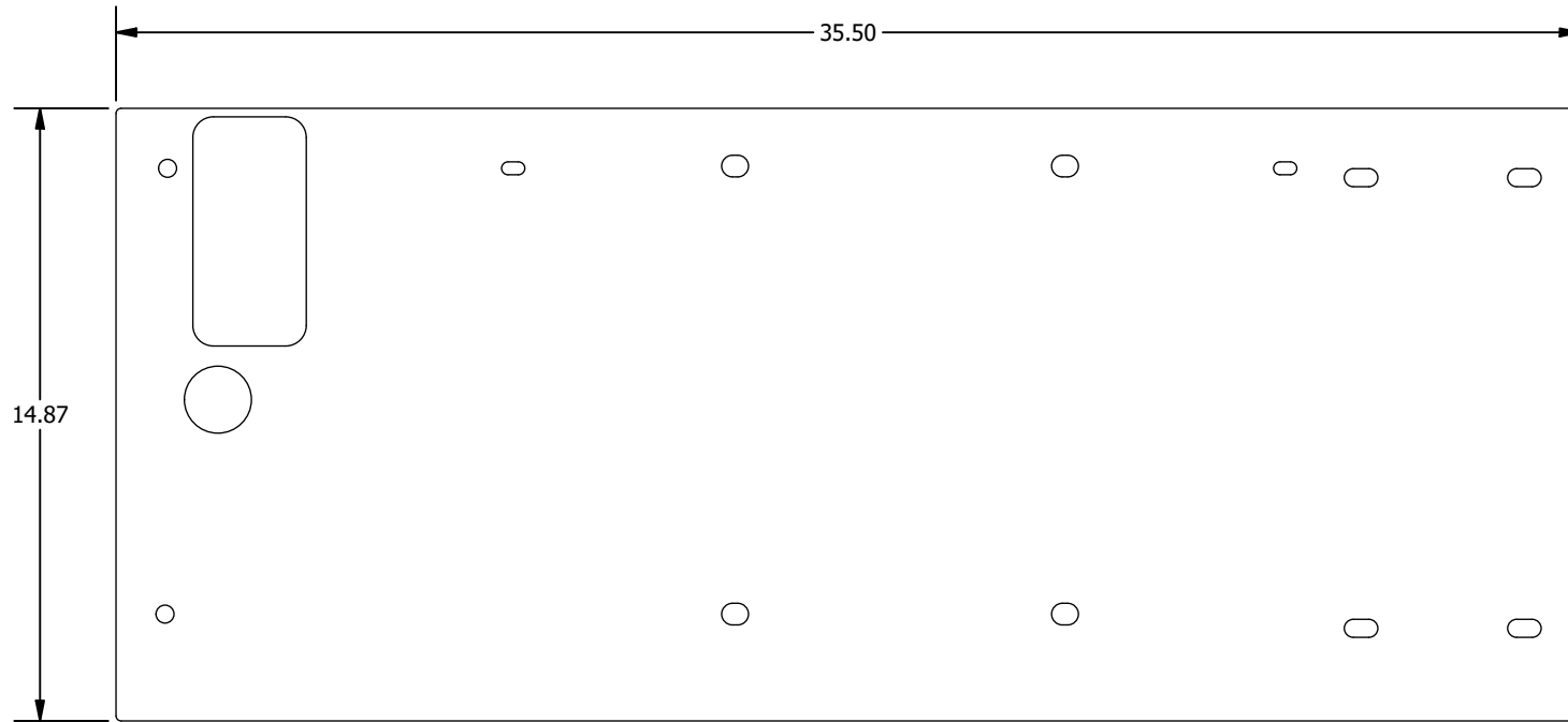
#MB1052 TAILGATE ARMOR QTY 1
