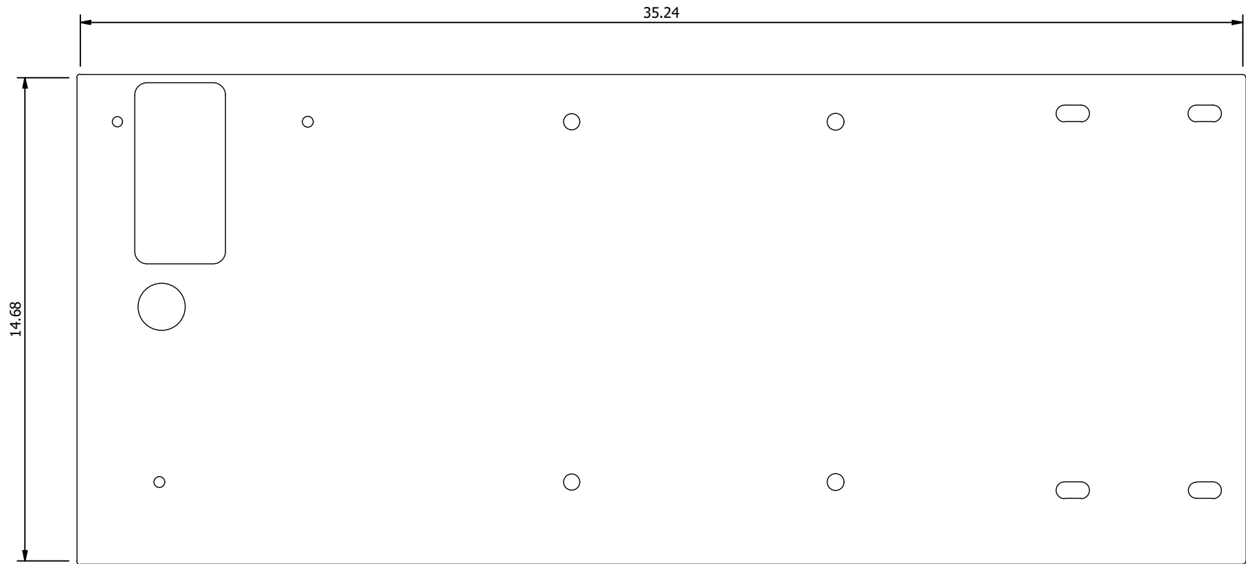
#MB1046 TAILGATE ARMOR QTY 1
