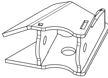
MB3041 - PASSENGER Qty: 1
