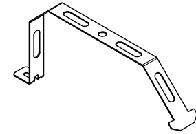
MB5040-09 TANK STRAP Qty: 1
