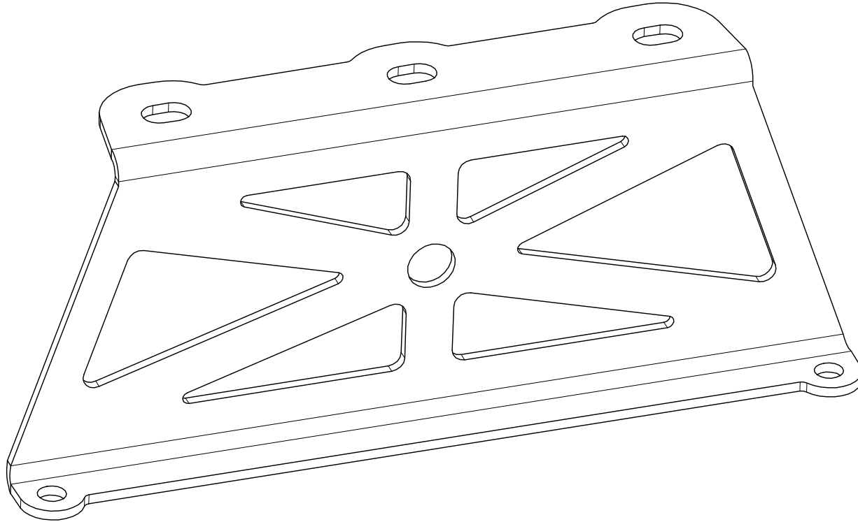
MB5009-01 Qty: 2
