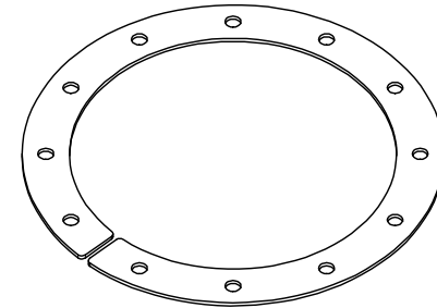
MB5007-03 Qty: 1
