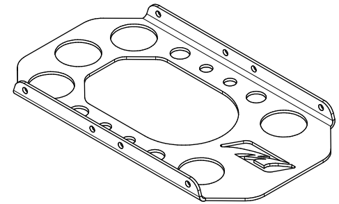
#MB5004-02 TOP PLATE QTY 1
