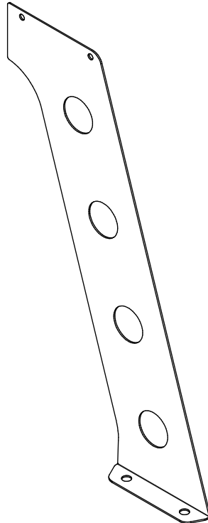
#MB5004-03_MIR/#MB5004-04 SIDE PLATE QTY 2
