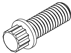
12 Point Bolt (Inches) 5/16\"-18 x 1-1/4\" Long Qty 10
