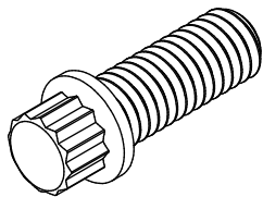
12 Point Bolt (Metric) M8 x 1.25 x 25mm Long Qty 14
