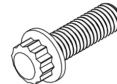
12 POINT BOLT M8-1.25mm x 25mm Qty: 12
