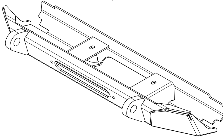
#MB3034 TJ/LJ FRONT HALF KIT BUMPER QTY 1
