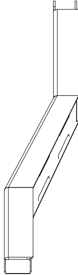
MB3025 - Weldment 02 Driver Frame Rail Qty: 1
