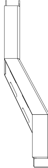
MB3025 - Weldment 04 Passenger Frame Rail Qty: 1
