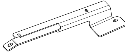
MB2152-03_MIR Qty: 1
