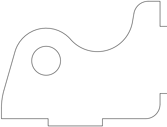
#MB1516-01 SHOCK MOUNT TAB QTY 4
