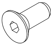
FLAT SOCKET SS 5/16"-18 x 3/4" QTY: 22
