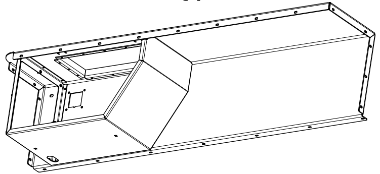
MB1185 - Weldment, Inner Fender Passenger Qty 1
