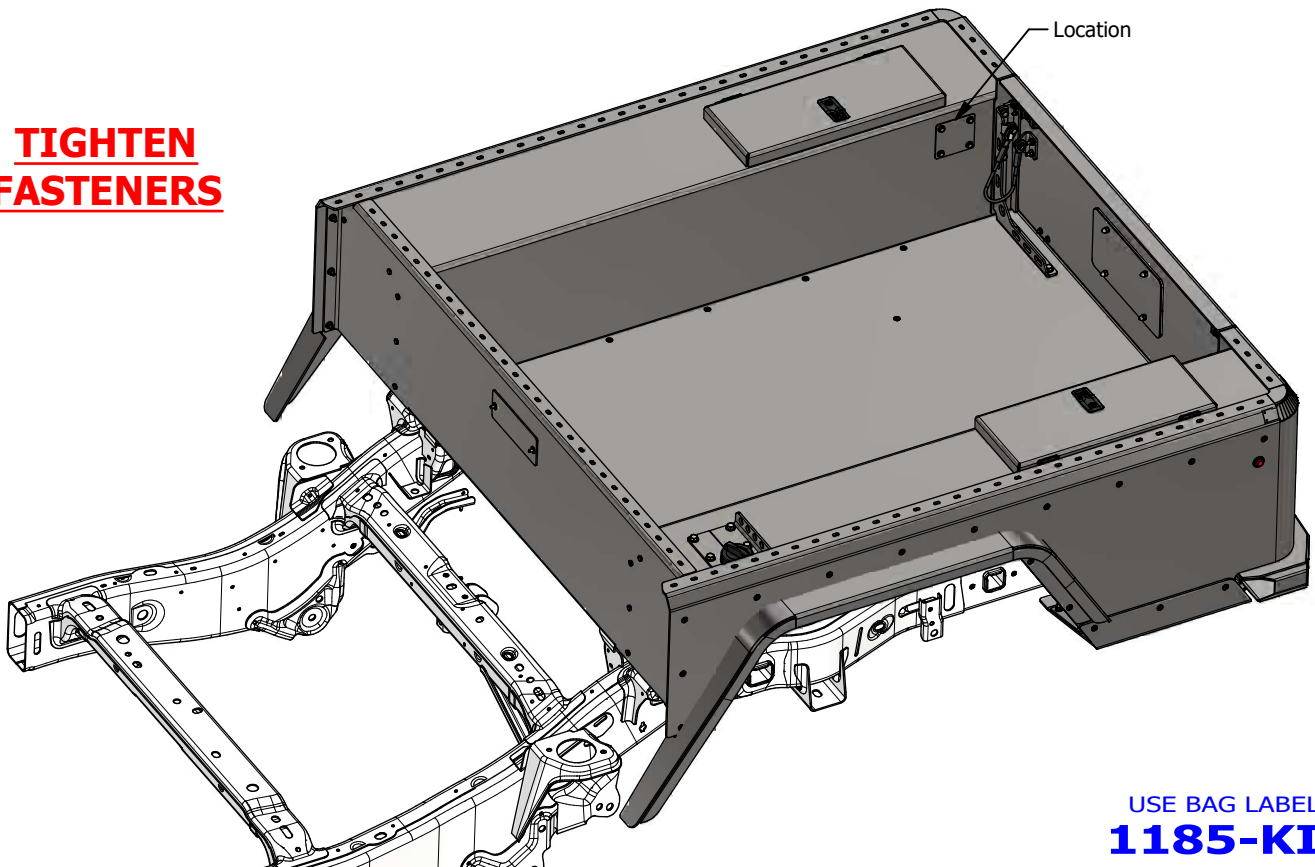
COVER PLATE ASSEMBLY
