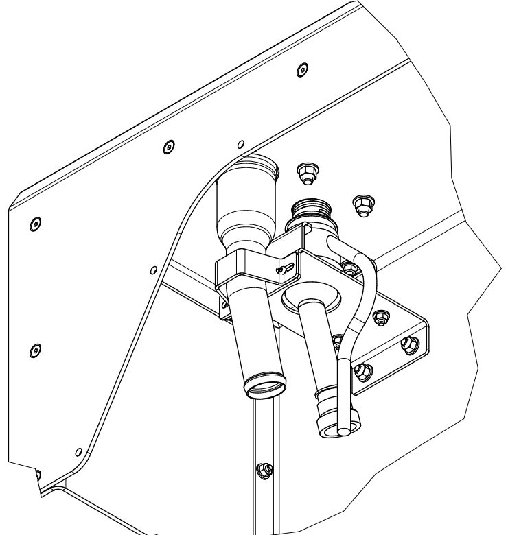
DIESEL ARRANGEMENT
