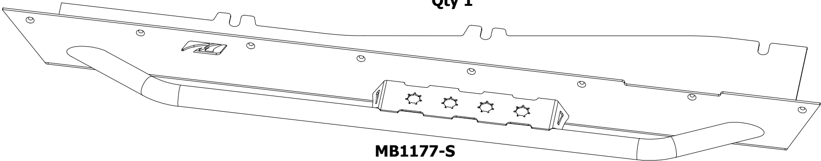
MB1177-S Weldment, Driver Qty 1
