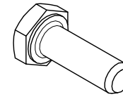
HEX HEAD BOLT 1/4"-20 x 0.75" Qty: 8
