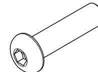
HEX BUTTON HEAD 1/4"-20 x 1" L, SS Qty: 4
